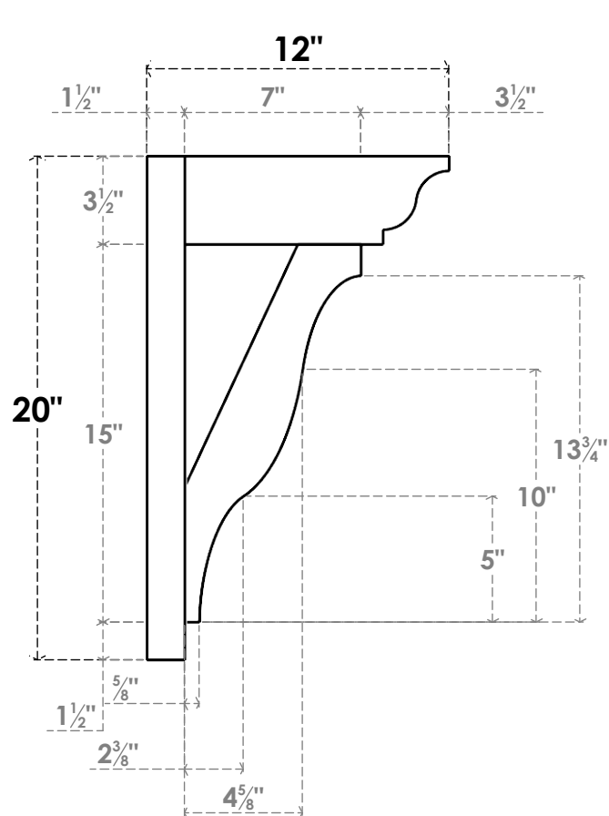
SIDE PROFILE
